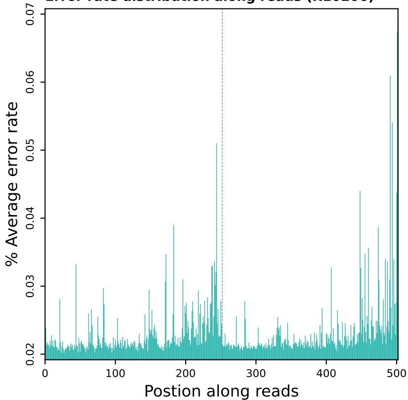
Error rate distribution along reads (R10206)
